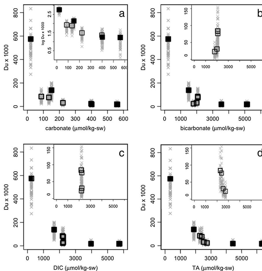
Figure 2. The D_U ( \text{Log } D_U ) versus (a) carbonate, (b) bicarbonate, (c) DIC, and (d) TA in \mu\text{mol/kg-sw} . Grey crosses represent individual laser-ablation measurements, whereas squares indicate mean values. Open squares represent data from acid/base manipulation and closed squares from pH-stable manipulation. Figures 2a–2d contain data of all treatments combined. Inset in Figure 2a depicts \text{Log } D_U versus carbonate ( \mu\text{mol/kg-sw} ). Insets in Figures 2b–2d represent data from the acid/base manipulation only; labeling for x and y axes is the same as in Figures 2b–2d and has been omitted. Please note that depiction of treatments A1 and B3 overlaps in Figure 2a (nearly identical D_U values at a carbonate ion concentration of approximately 400 \mu\text{mol/kg-sw} ).
